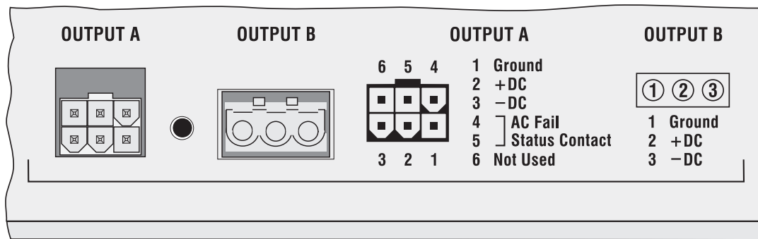
Figure 5. Front view of Model 738 cabinet showing 6-position connector and 3-position terminal strip
