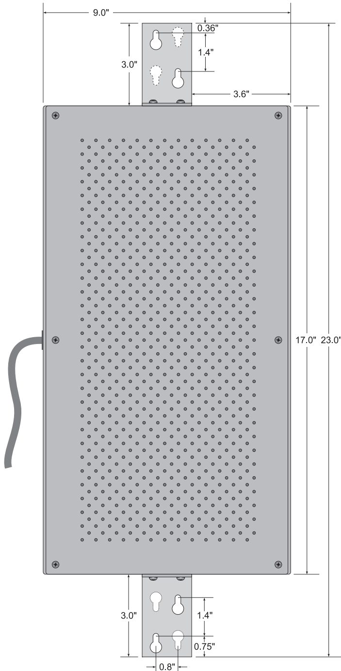
Figure 4. Recommended Model 738 wall-mounting configuration
