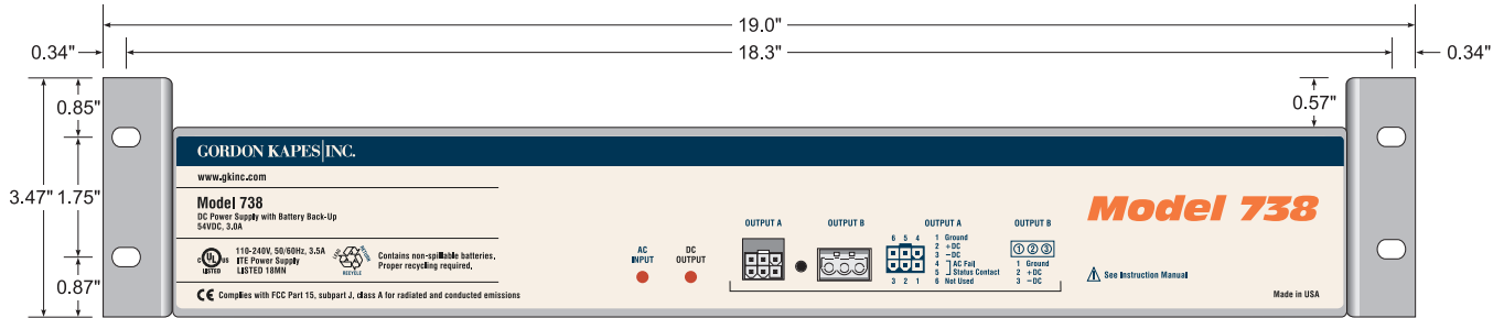
Figure 2. Front view of Model 738 cabinet showing 19-inch flush rack-mount brackets attached
